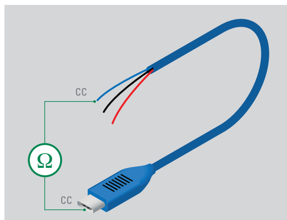
Figure 10. USB Type-C to open cable quality assurance test
