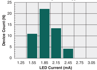
Typical I F for Switch Operation (N=50, I L =150mA DC )
