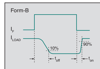
Switching Characteristics of Normally Closed Devices
