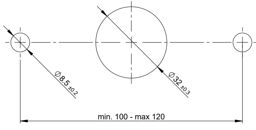
Fixing holes
