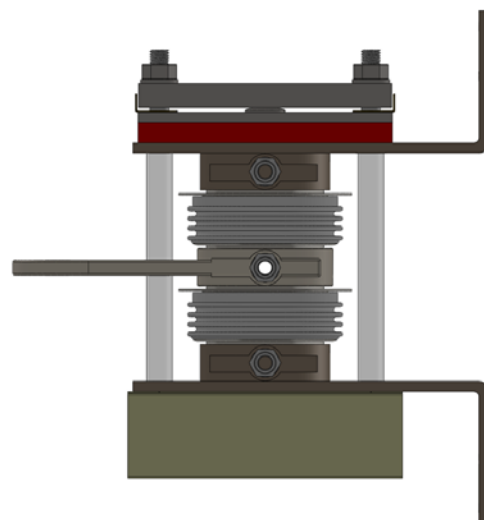
Step 8: The assembly is now complete.
