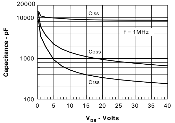
Figure 8. Capacitance Curves
