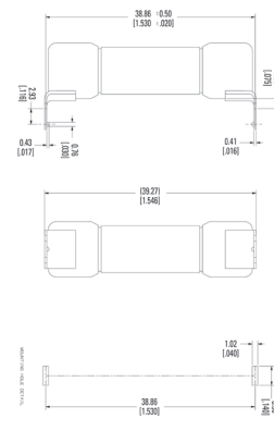
ZXPCL PCB Mount (Long)
