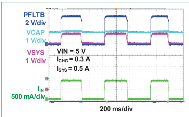
Fig9 : Charger 4VIN Switch to 5VIN (Setting VIN_UVLO 4.1 V)
