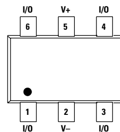
SP724 (SOT-23) TOP VIEW
