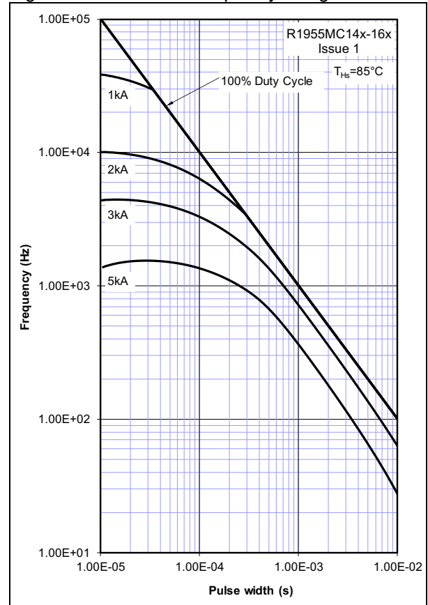
Figure 12 - Sine wave frequency ratings
