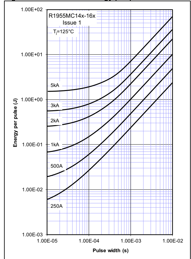
Figure 10 - Sine wave energy per pulse
