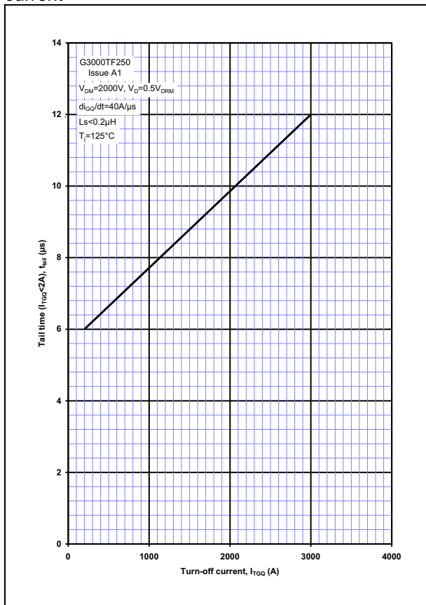
Figure 15 – typical tail time ( I_{TQ}<2A ) vs. turn-off current
