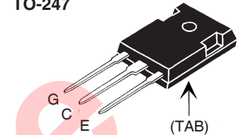
TO-247
