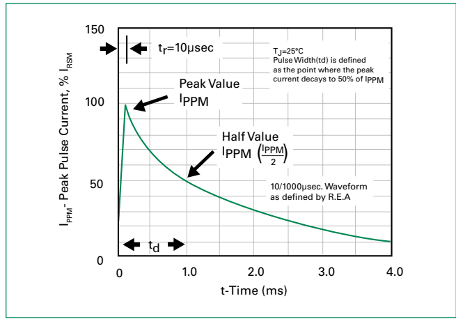
Figure 4 - Pulse Waveform
