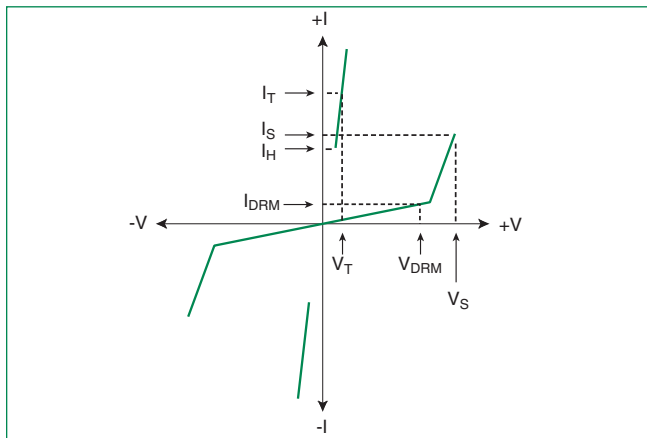
V-I Characteristics
