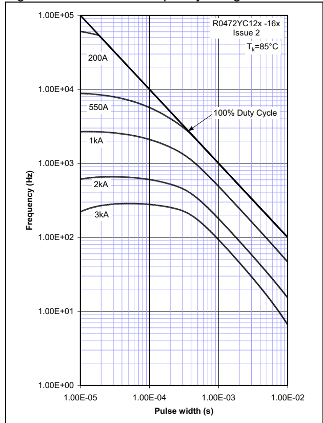
Figure 14 - Sine wave frequency ratings
