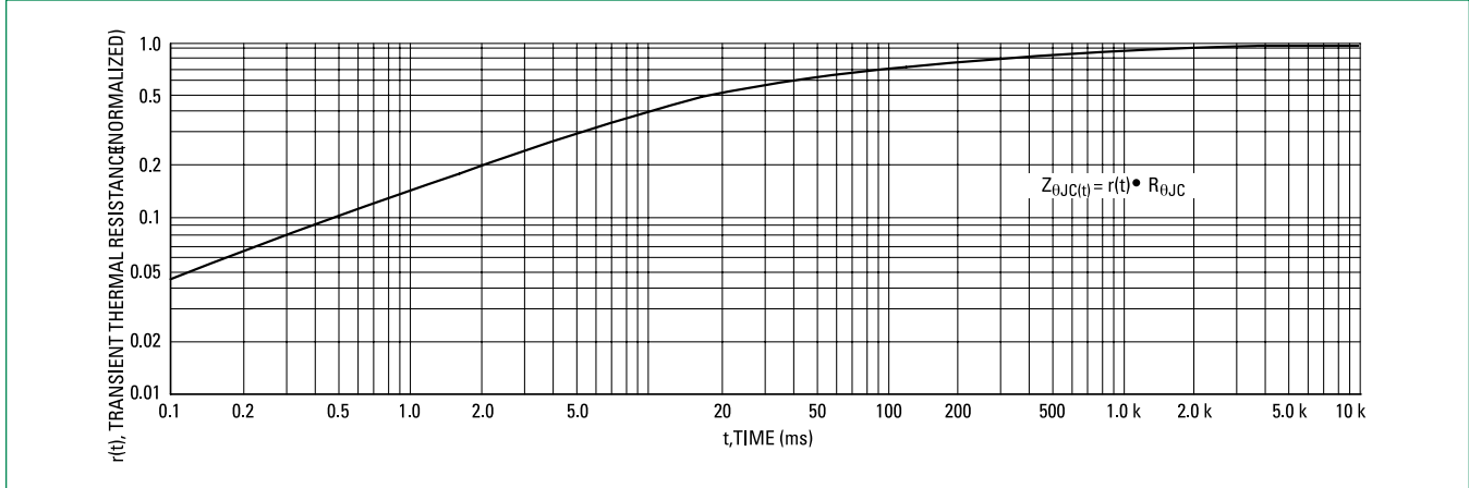
Figure 10. Thermal Response
