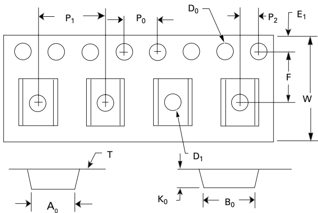
Tape Specifications
