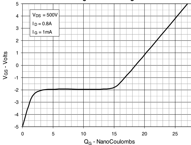
Fig. 14. Gate Charge
