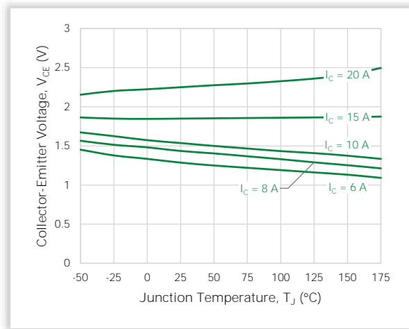
Figure 4. Collector-Emitter Voltage vs. Junction Temperature
