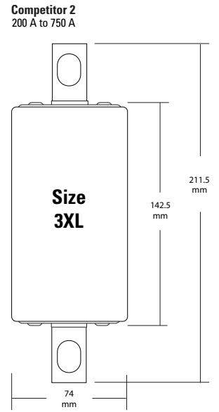
Comparable Current Rating in a Smaller Case Size
