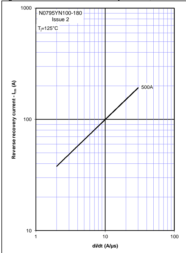
Figure 7 – Peak Reverse Recovery Current, I_{rm}
