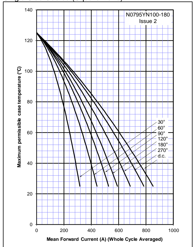
Figure 16 – On-state current vs. Case temperature – Single Side Cooled (Square wave)
