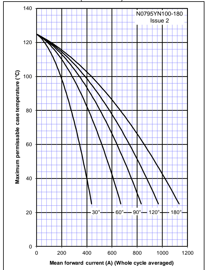
Figure 12 – On-state current vs. Case temperature – Double Side Cooled (Square wave)
