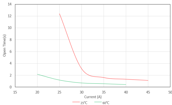
Open Time vs. Current Curves – @ 25°C & 60°C
