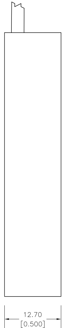
SIDE VIEW
