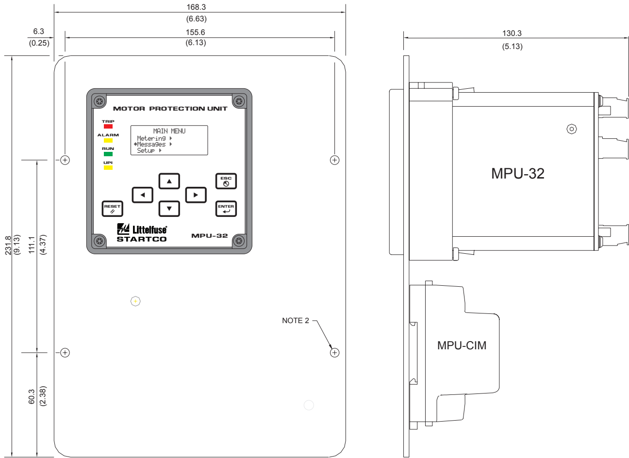
TYPICAL CONFIGURATION
